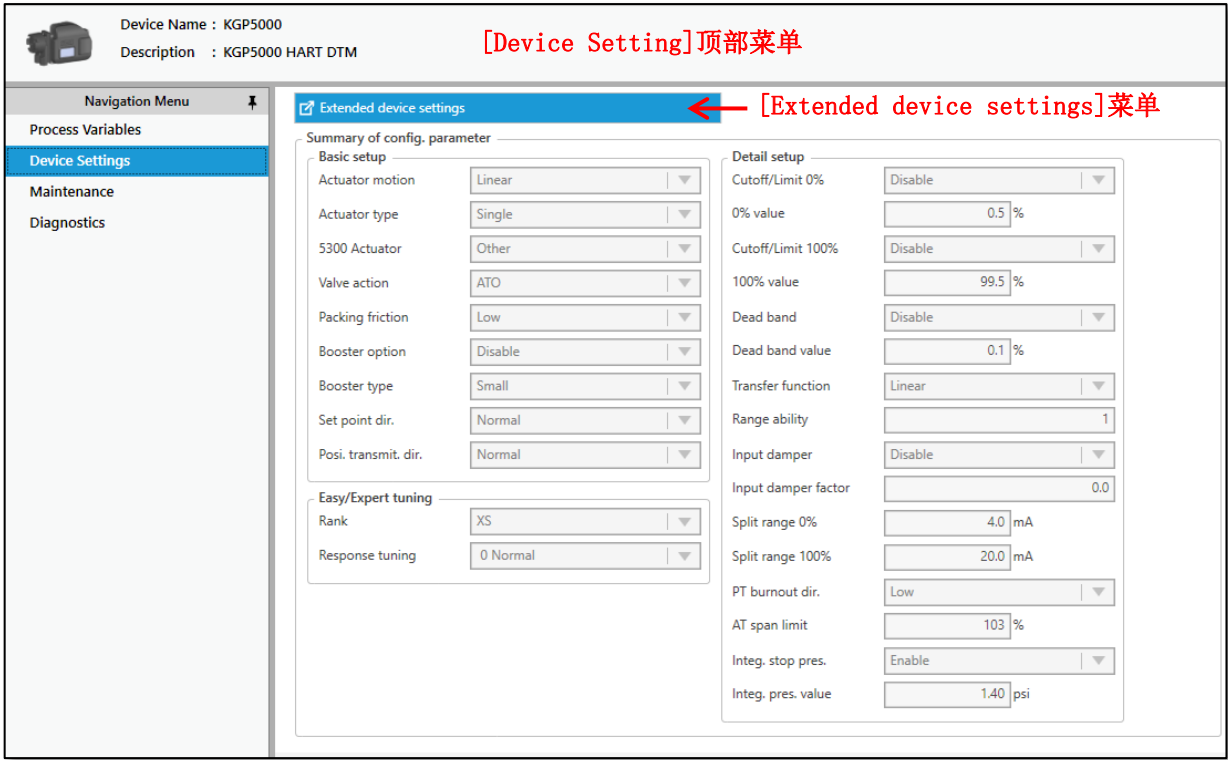
图 2. 2. 2a [Device Settings]顶部菜单
