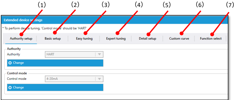
图 2. 2. 2b [Extended device settings]菜单
