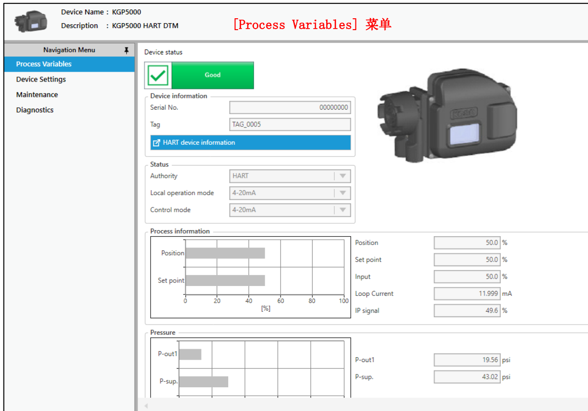
图 2.2.1a [Process Variables] 菜单
