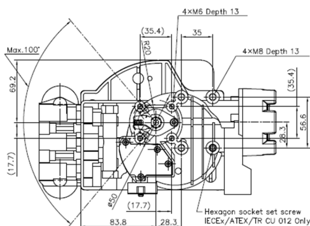
A VIEW
